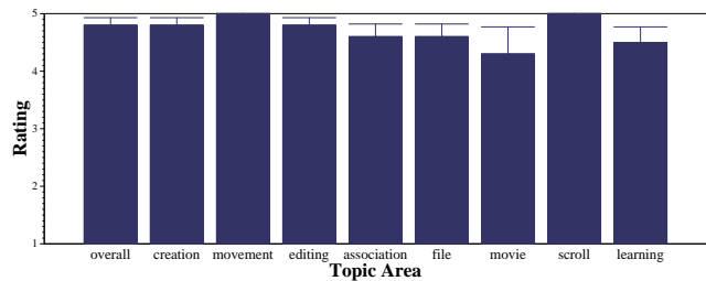
Figure 3. Novice user evaluation results, broken down by topic area. Each rating is on a five point Likert scale, ranging from "Difficult" (1) to "Easy" (5). Error bars display standard errors of the mean.
