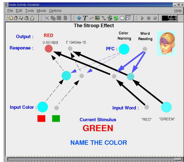
Figure 2. The main NAV window displaying an animation of a model of the Stroop task. Node activity is reflected in both the size and color of nodes, and textual labels are dynamic.
