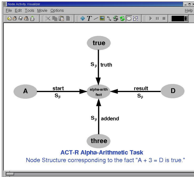
Figure 1. The main NAV window displaying an animation of a component of the spreading activation based memory network of an ACT-R model.
